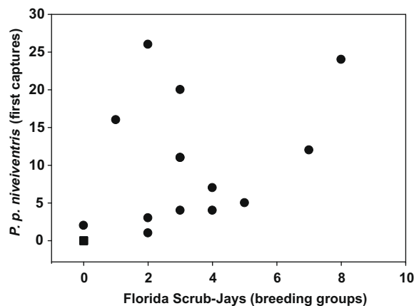
Fig. 4. Relationship between the number of Florida Scrub-Jay breeding groups and first-time captures of Peromyscus polionotus niveiventris in management compartments at Cape Canaveral Air Force Station, Florida. Data on Florida Scrub-Jay breeding groups are from Stevens and Knight (2004). Square symbol represents five compartments.
